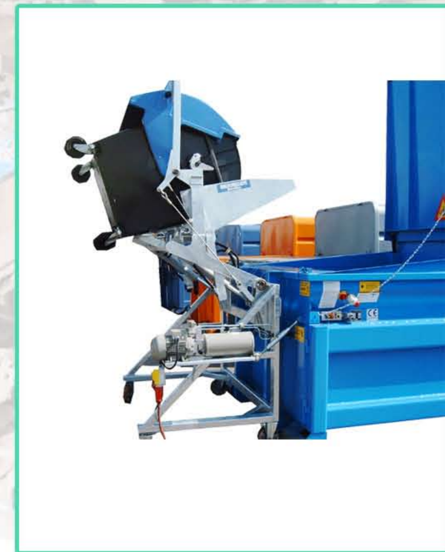
Hydraulic Mobile Bin Lifter
